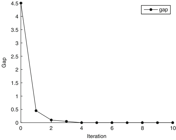
Fig. 6.3 Convergence of the descent algorithm, which is terminated with the gap less than 10^{-10}
