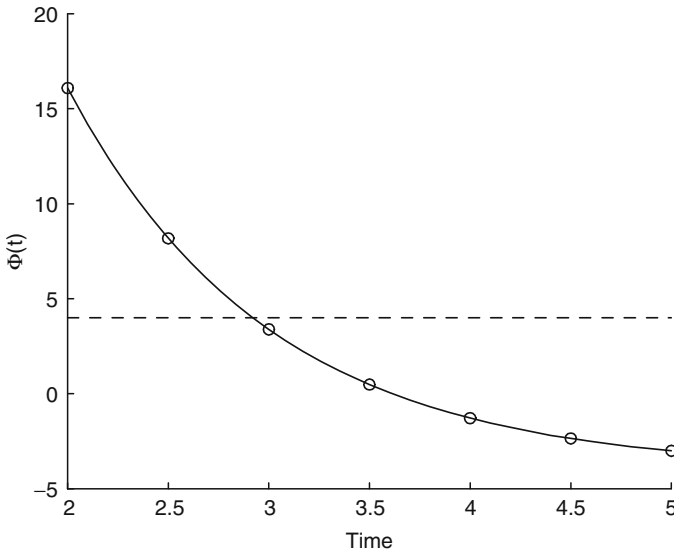
Fig. 3.2 Plot of the control law
