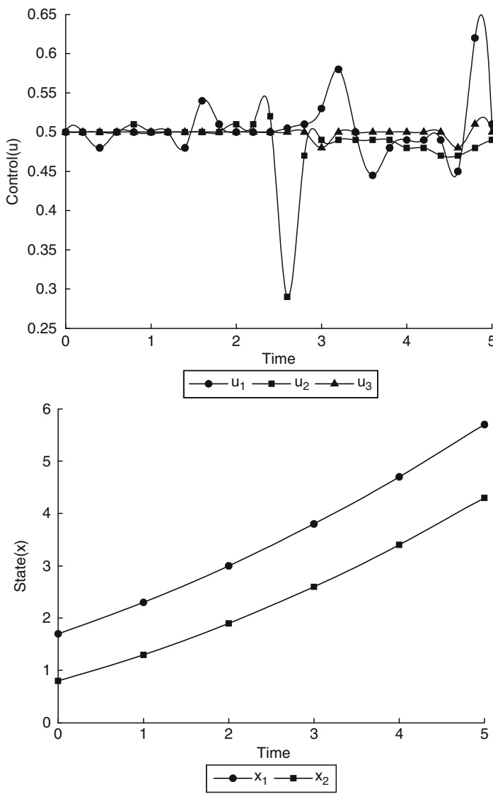
Fig. 6.6 u^* vs. time and x^* vs. time without time shifts
