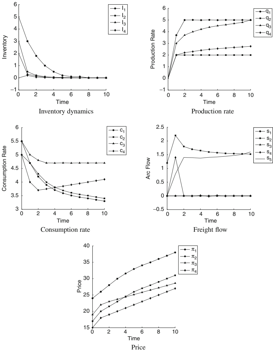
Fig. 8.2 Solution by discrete-time approximation
