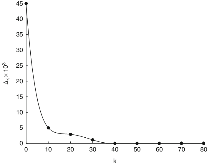
Fig. 9.8 Control fluctuations from one iteration to the next: (\Delta_k) vs. the iteration counter (k)
