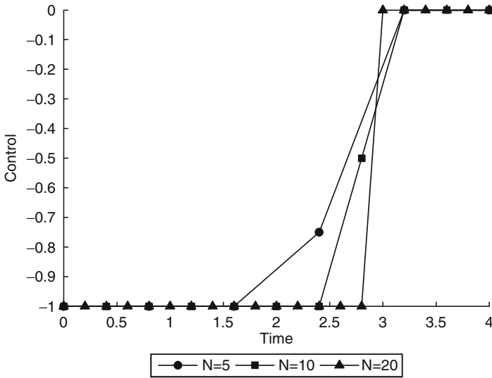
Fig. 3.4 Optimal control trajectories with different levels of time resolution
