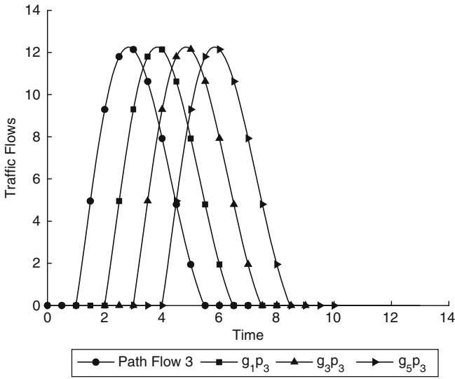
Fig. 9.4 Path and arc exit flows for path p_3
