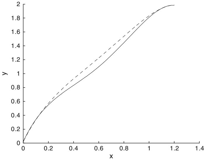
Fig. 3.1 An Approximate solution of the brachistochrone problem
