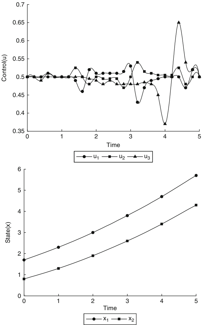
Fig. 6.5 u^* vs. time and x^* vs. time with fixed time shifts
