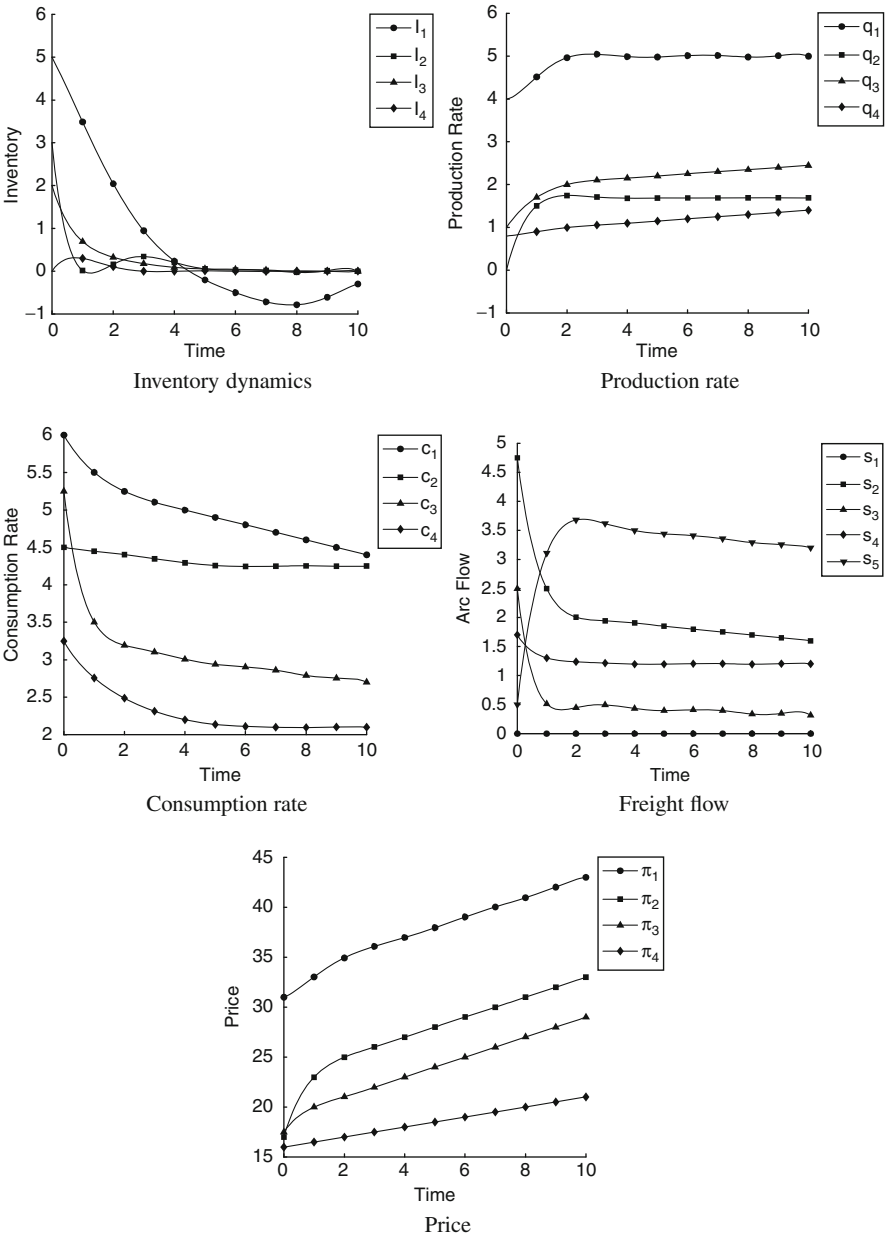
Fig. 8.3 Solution by continuous time gradient projection method
